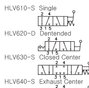
HLV610-S Single
